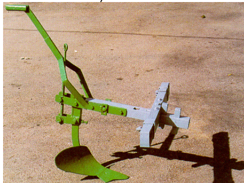
Light Mould Board Plough
